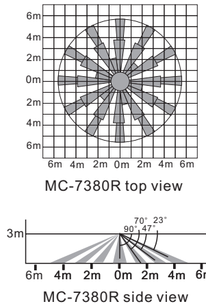
MC-7380R side view
