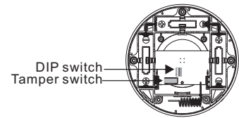
Figure 2. Inside View
